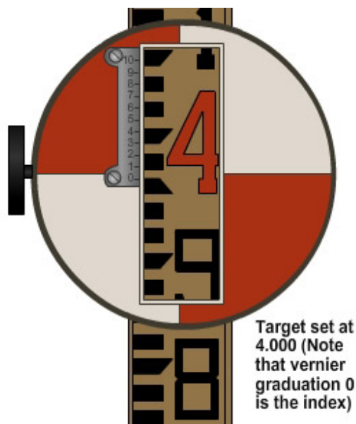
Figure 5-23 – Target.
