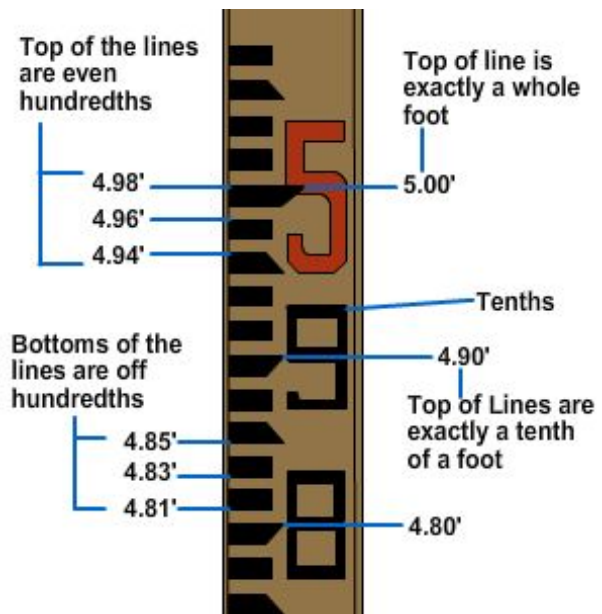
Figure 5-21 – Philadelphia rod marking.
