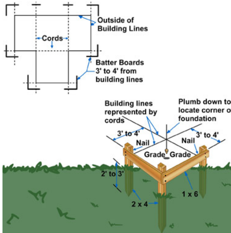
Figure 5-28 – Batter boards.
