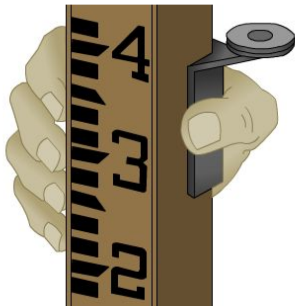
Figure 5-25 – Bull's eye rod level.
