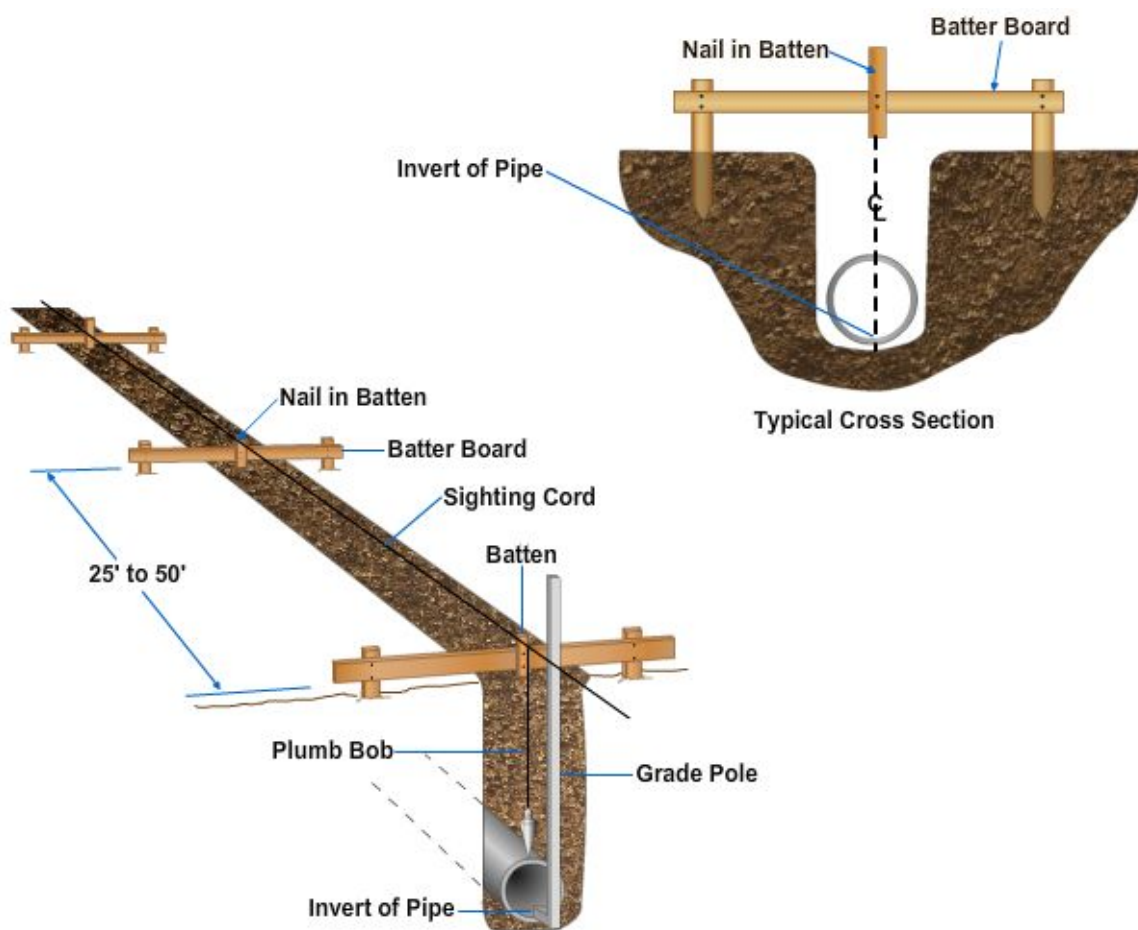
Figure 5-29 – Use of batter boards (with battens) for utility stakeout.
