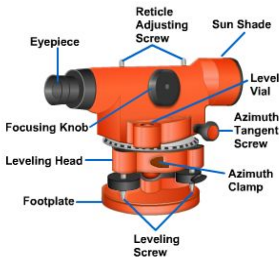
Figure 5-13 – Dumpy level.
