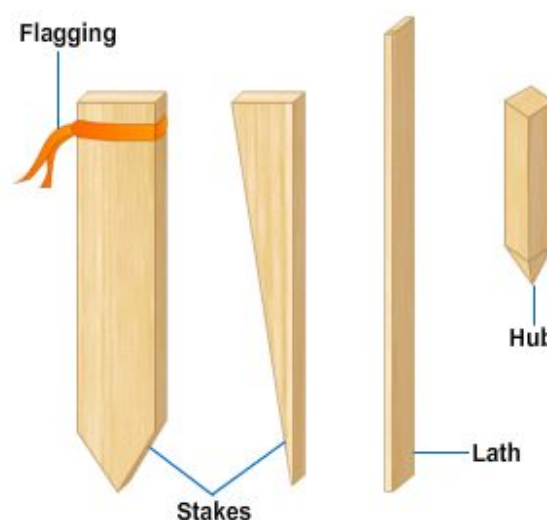
Figure 5-31 – Types of stakes.
