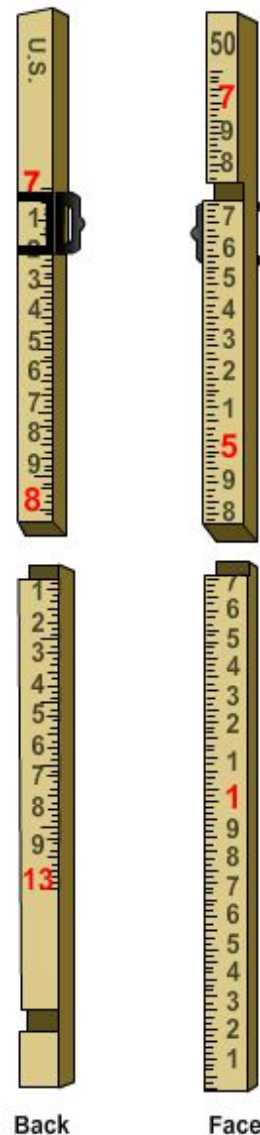
Figure 5-19 – Back and face of Philadelphia leveling rod.
